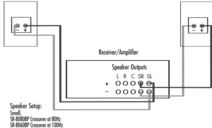
Figure 3 – Connecting Speaker to Amplifier
